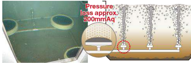
Disc-type diffuser
