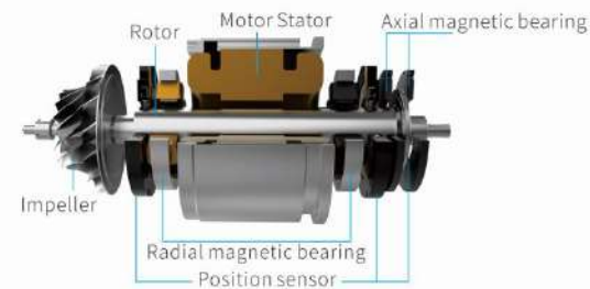
Rotor and impeller are connected directly energy saving and consumption reduction
