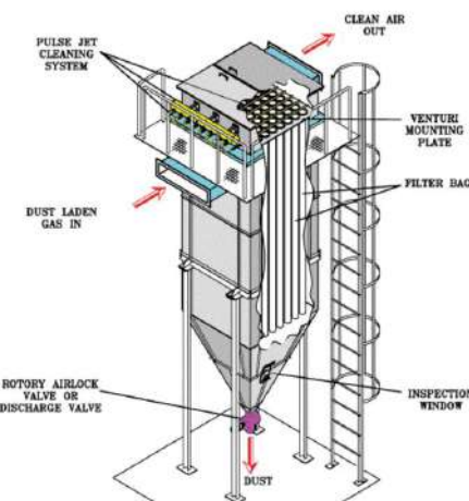
(PULSE JET TYPE) BAG FILTER
